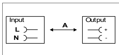
Fig. 17-1 Dielectric strength
