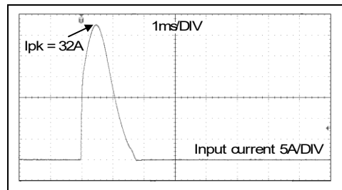
Fig. 5-2 Zoom into the first inrush peak
