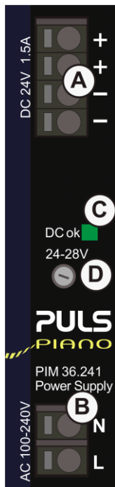
Fig. 10-1 Front side
