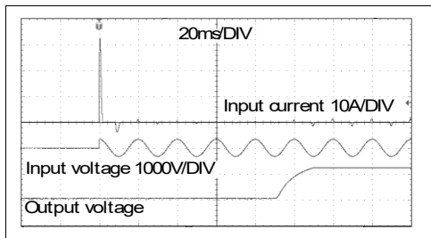
Fig. 5-1 Typical turn-on behavior at 230Vac and 25°C ambient
