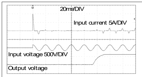
Fig. 5-3 Typical turn-on behavior at 120Vac and 25°C ambient
