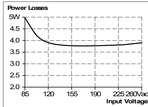
Fig. 8-4 Losses vs. input voltage at 24V, 1.5A, typ.
