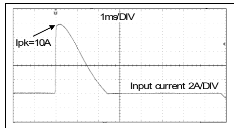
Fig. 5-4 Zoom into the first inrush peak
